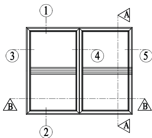
TYPICAL ELEVATION
