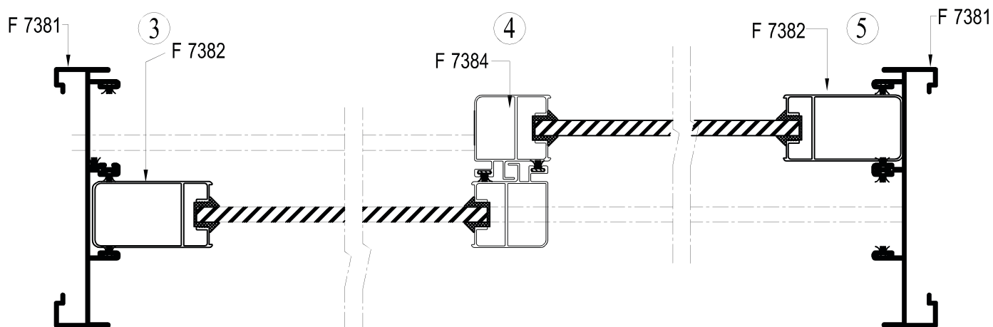
SECTION B-B
