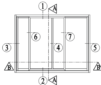
TYPICAL ELEVATION
